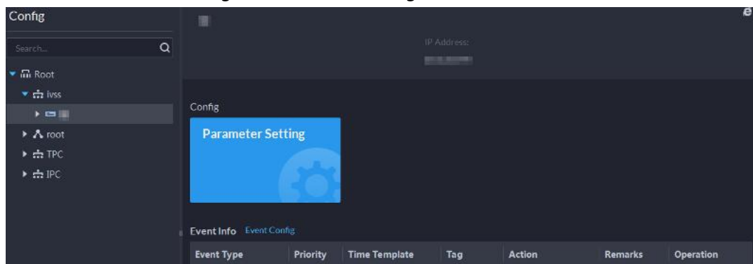
Figure 3-55 Device configuration
