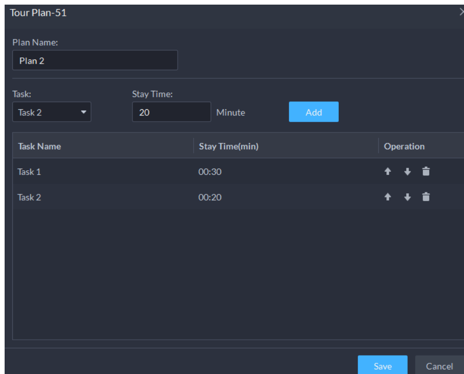
Figure 5-50 Tour plan
