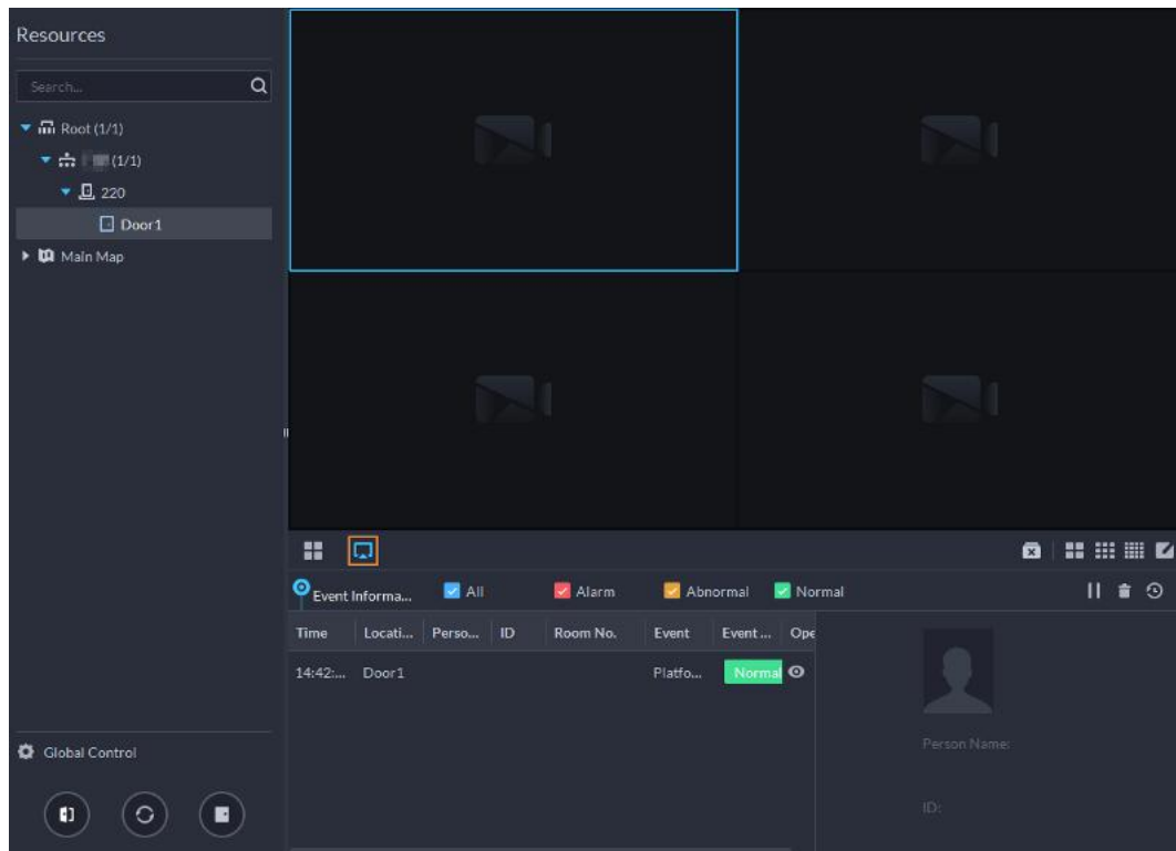
Figure 5-74 Viewing video (2)
