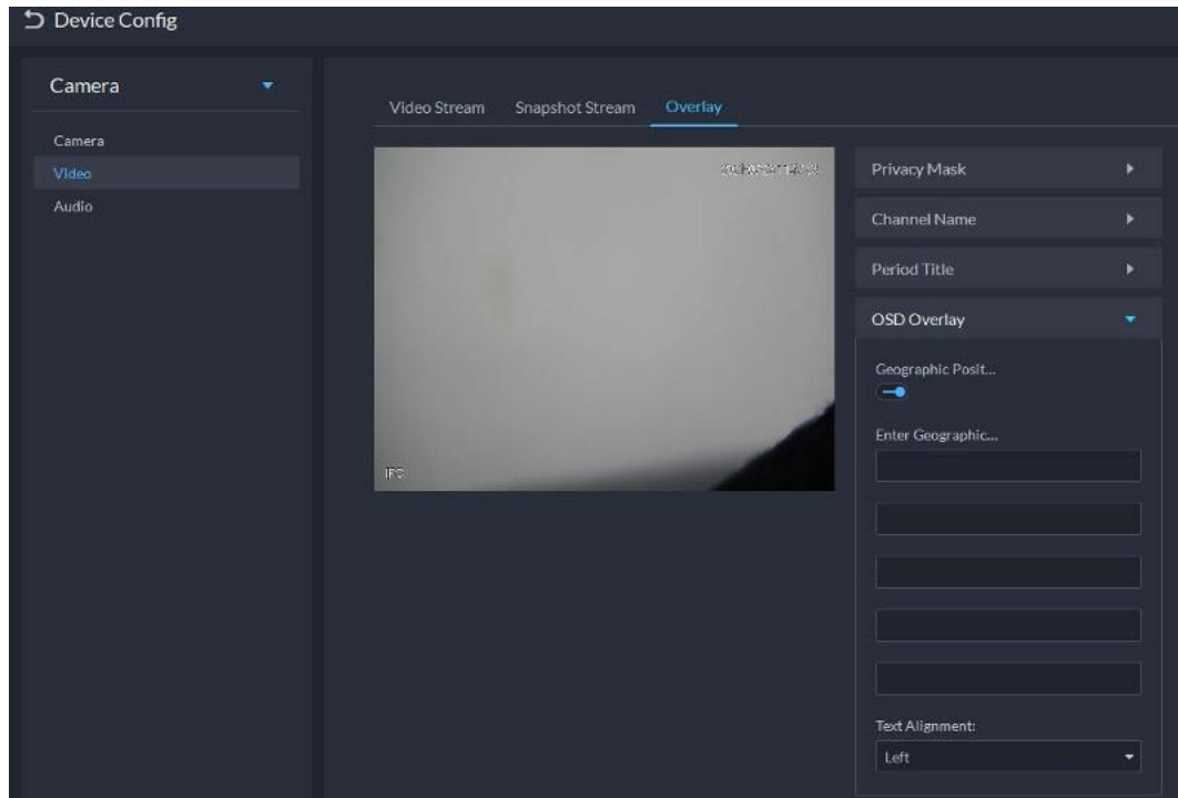
Figure 3-54 OSD overlay
