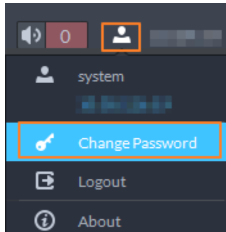
Figure 3-62 Change password
