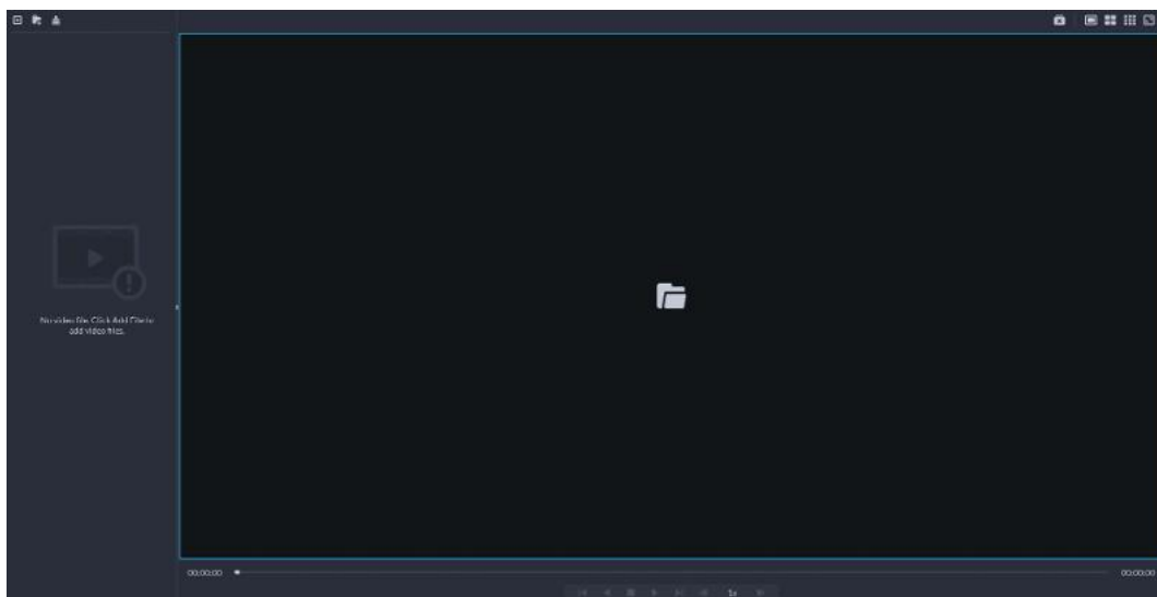
Figure 8-8 Local video
