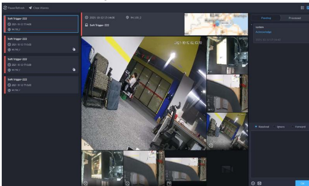
Figure 5-56 Alarm details
