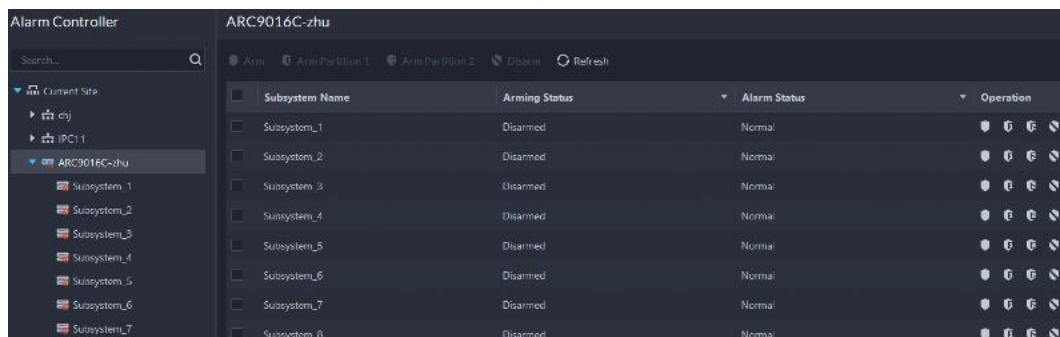
Figure 5-62 Subsystems
