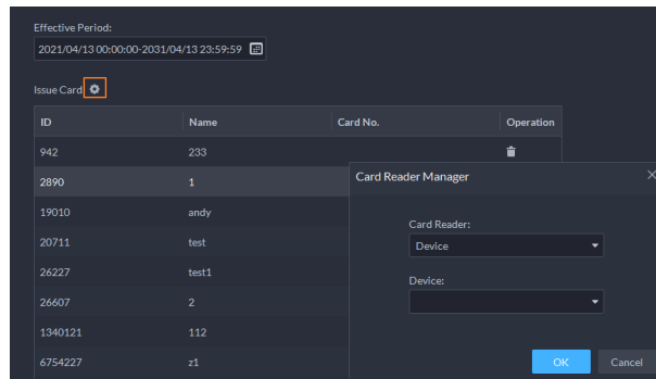
Figure 4-38 Reader manager
