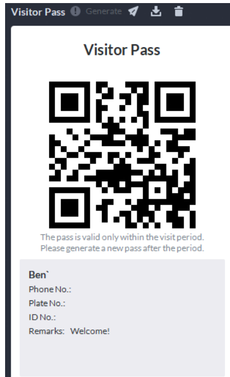
Figure 5-89 Authentication
