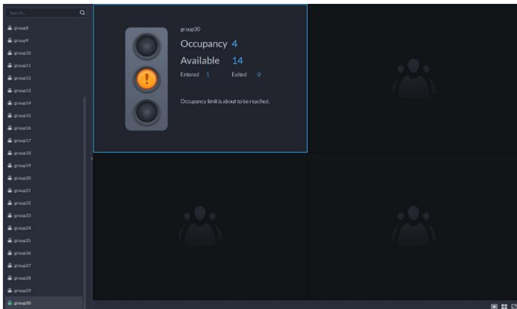
Figure 5-97 Real-time count
