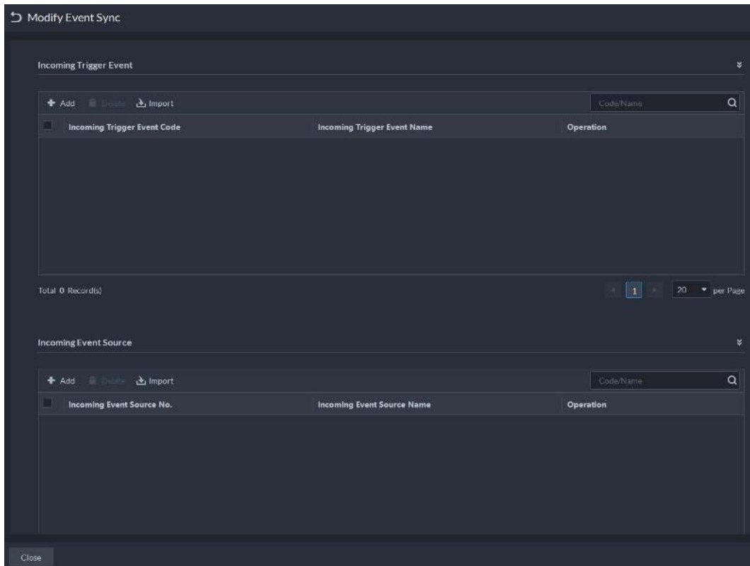
Figure 4-82 Synchronize events
