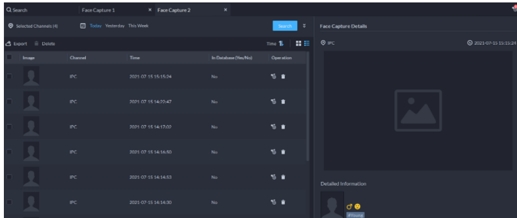
Figure 5-67 Search result
