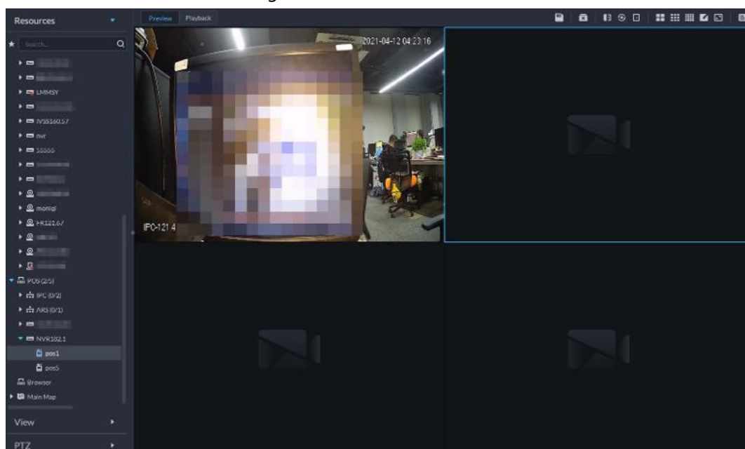
Figure 6-9 POS video
