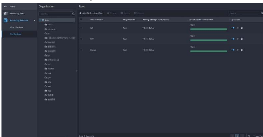
Figure 3-28 File retrieval
