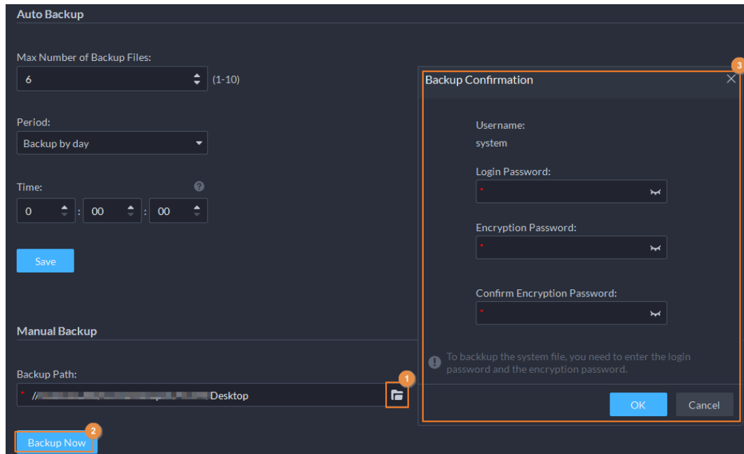
Figure 7-16 Manual backup
